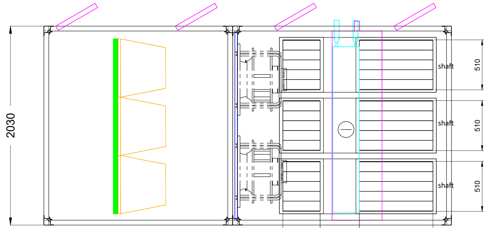
Top View
